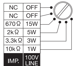
[Impedance Selection]
