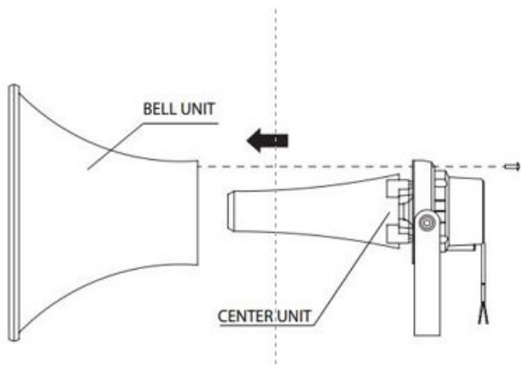
Horn Speaker 50W ZH-5050M-AS (Dengan Transformer)
