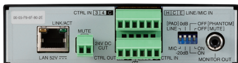
IP-A1PG rear
