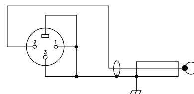
Plug Diagram
