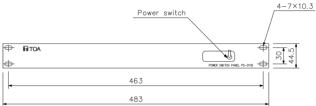
Front View
